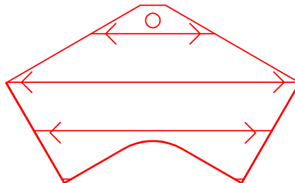
STANDARD LAMINATE DIRECTION FOR 120 DEGREE SURFACES
